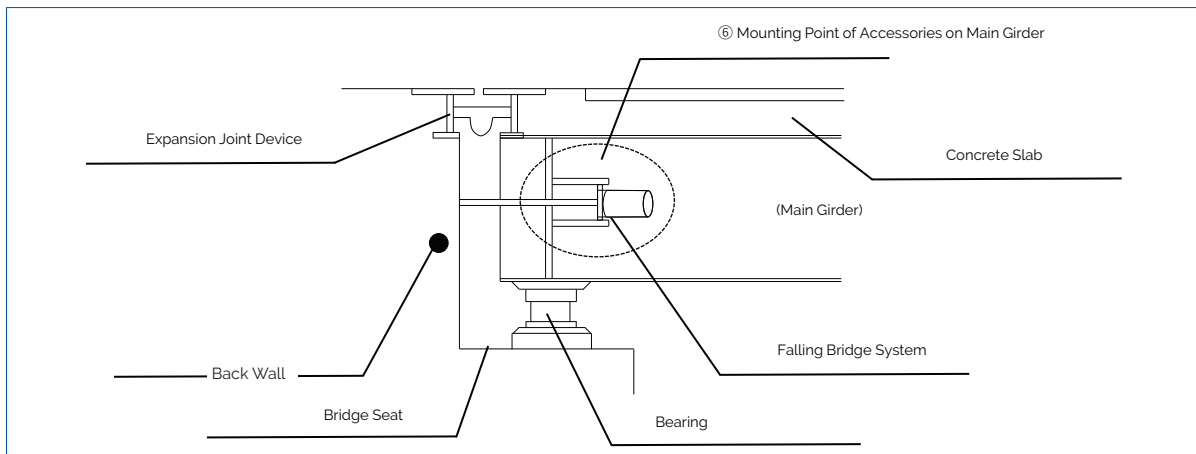
Figure 3.11 Girder end
