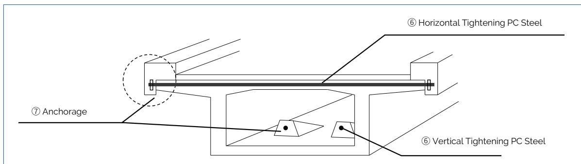
Figure 3.6 PC box girder bridge
