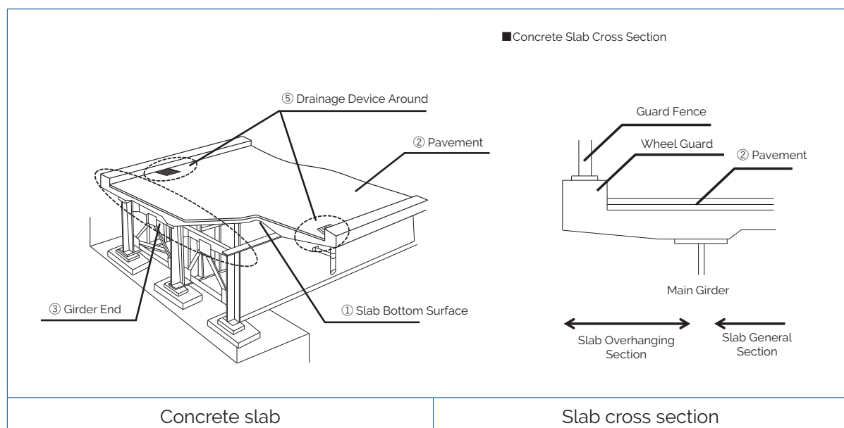
Figure 3.8 Concrete slab
