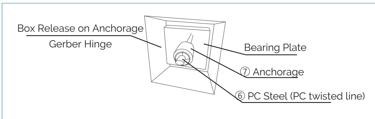
Figure 3.3 Anchorage on PC steel
