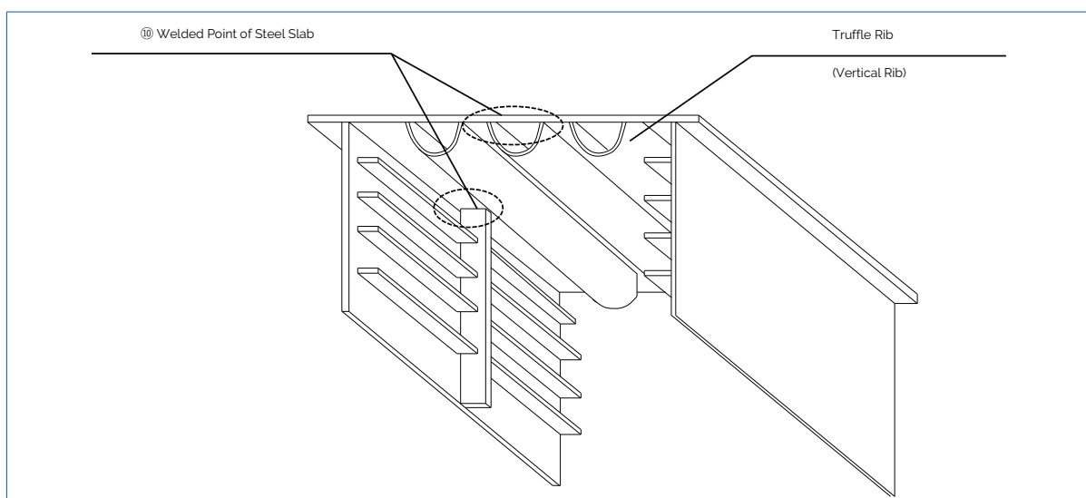
Figure 3.15 Steel slab
