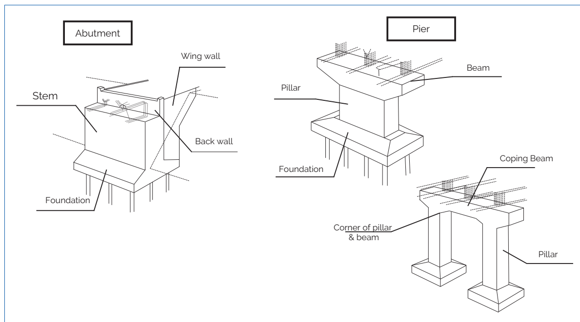
Figure 3.16: Abutment and pier
