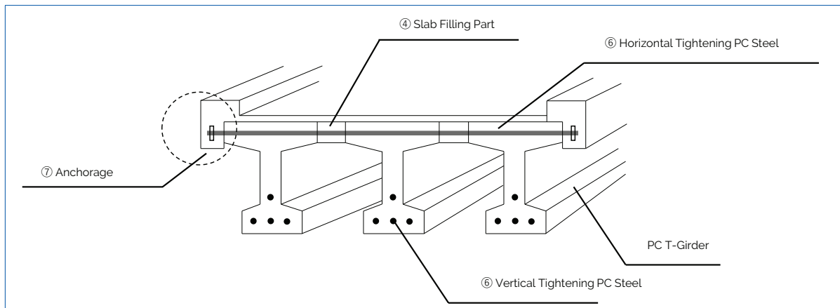
Figure 3.5 PC T-girder bridge
