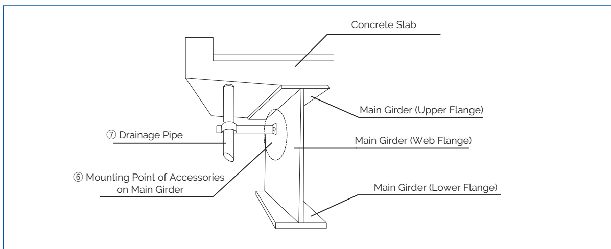
Figure 3.12 Vicinity of drainage device
