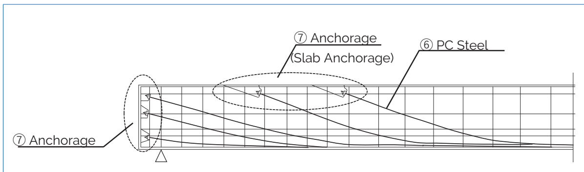
Figure 3.2 PC girder steel arrangement
