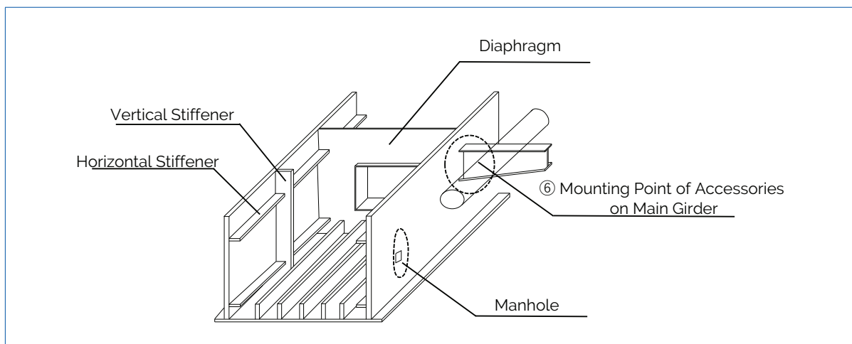
Figure 3.14 Inside box girder
